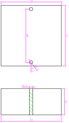
DC-DC Power Size (Inside)
